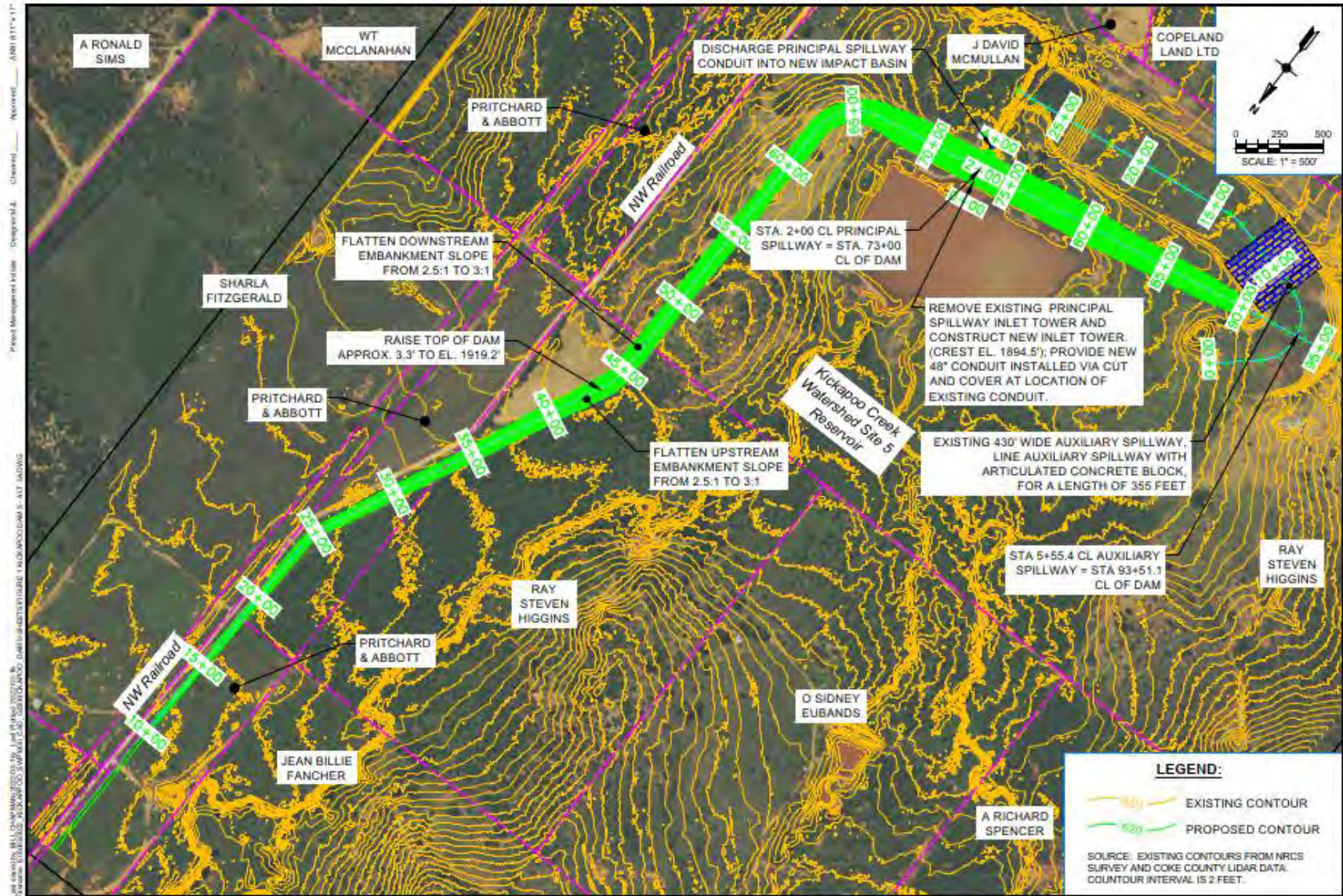
AECOM Figure: C-8 ALTERNATIVE 3 - HIGH HAZARD POTENTIAL REHABILITATION OF FRS No. 5
